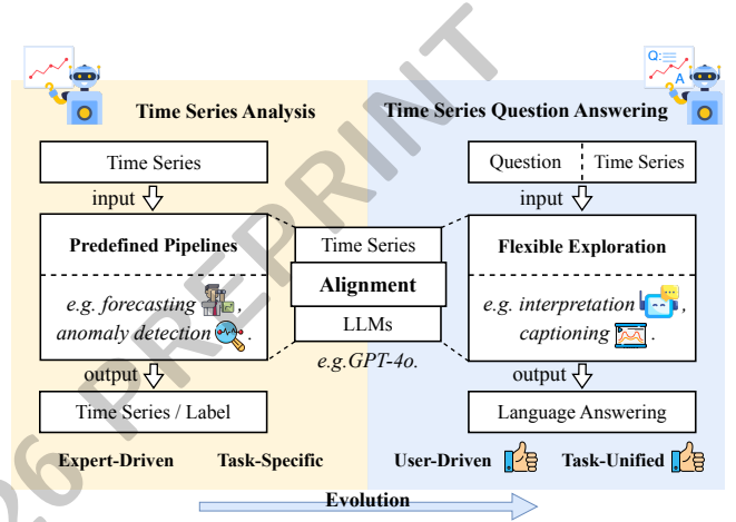
Figure 1: Comparison between Time Series Analysis and Time Series Question Answering under alignment of time series with LLMs.
