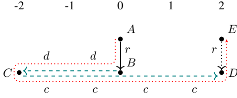
Figure 4: The word ddcccc read along the dotted line witnesses that \mathcal{T} \models A \subseteq \bigcirc^2 E .
