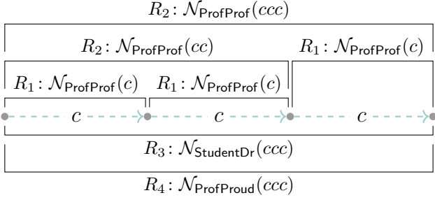
Figure 2: An illustration for the facts that c^3 \in LG_{\mathcal{T}}(\mathcal{N}_{\text{ProfProf}}) , in the upper part, and c^3 \in LG_{\mathcal{T}}(\mathcal{N}_{\text{ProfProud}}) , in the lower part. Each symbol c stands for a step forward in time. The grammar rule of G_{\mathcal{T}} used to obtain each proposition is given in the following denotation: R_1: \mathcal{N}_{\text{ProfProf}} \rightarrow c , R_2: \mathcal{N}_{\text{ProfProf}} \rightarrow \mathcal{N}_{\text{ProfProf}}\mathcal{N}_{\text{ProfProf}} , R_3: \mathcal{N}_{\text{StudentDr}} \rightarrow c^3 , R_4: \mathcal{N}_{\text{ProfProud}} \rightarrow \mathcal{N}_{\text{StudentDr}} .
