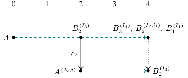
Figure 3: An illustration for \mathcal{T}_G \models A \sqsubseteq \circ^4 B_1 . The concept inclusion used for each inference is given in superscript (cf. Example 4).
