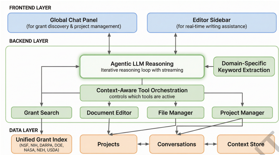
Figure 1: GRAIL system architecture: Frontend interface with chat panel and editor sidebar, agentic LLM reasoning with context-aware tool orchestration, and integrated data layer for grant indexing and project management.
