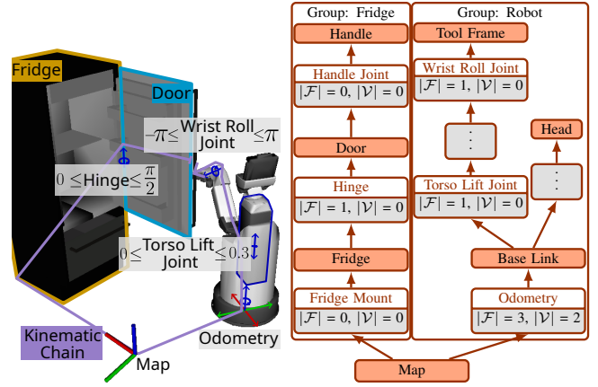
Figure 2: An example of a world containing a fridge and a Toyota HSR (left), with its kinematic model (right).
