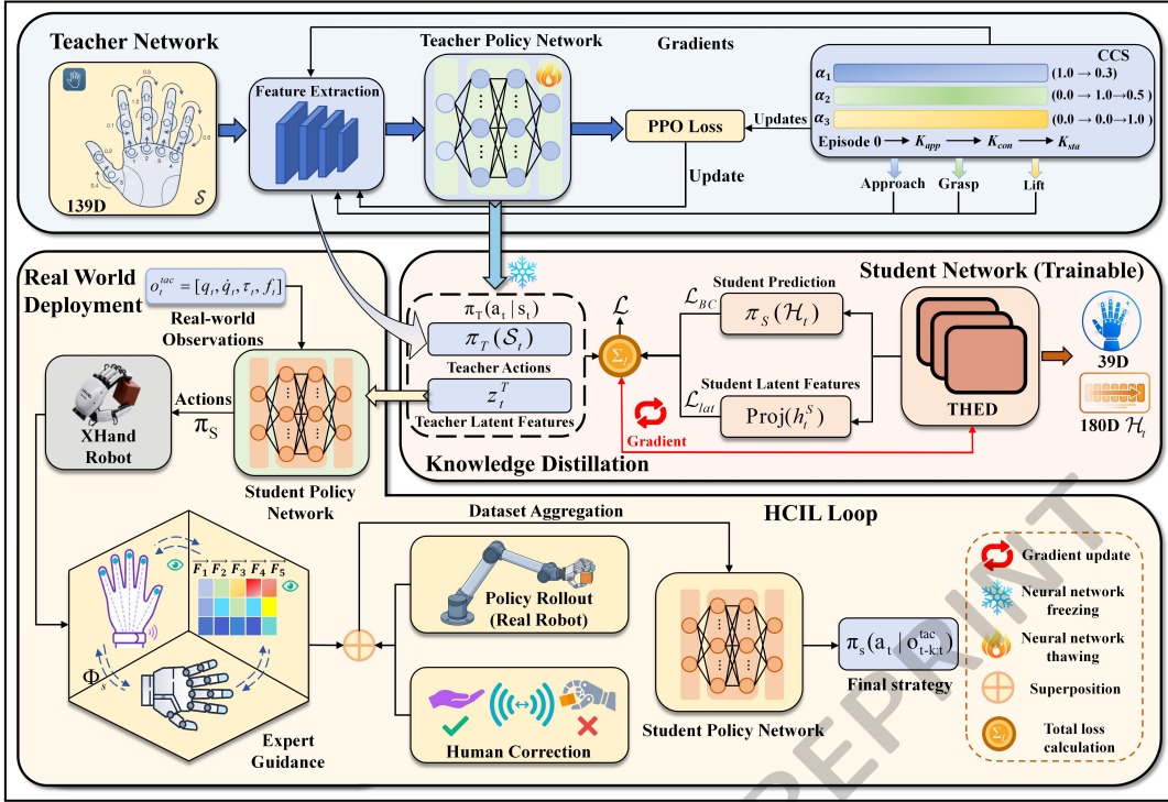
Figure 1: Flowchart of the PECHC algorithm framework. Note the ‘Failure-Triggered’ loop in HCIL, which activates only upon slip detection, significantly reducing human annotation cost compared to full-time teleoperation.
