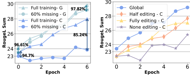
(a) Overall performance be- (b) Client (C) performance com- tween full and 60% missing parison among different editing modality training. strategies.
