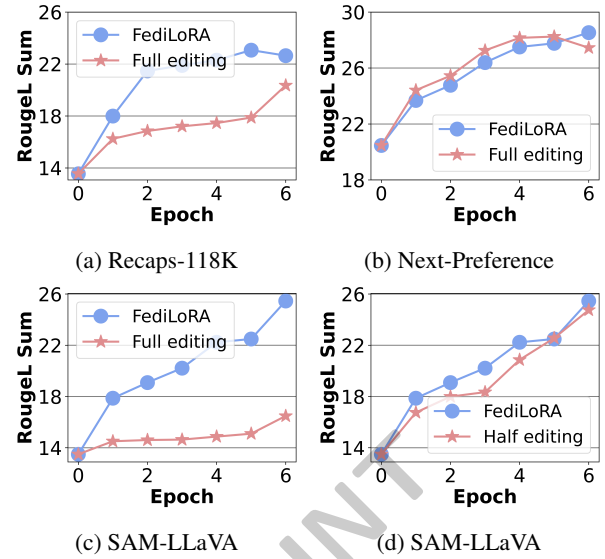
Figure 5: Comparing editing methods. (a), (b) and (c) present the performance comparison between full-editing and FedILoRA on three datasets respectively. (d) shows the comparison of half-editing and FedILoRA.
