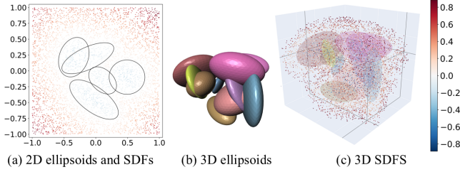
Figure 3: Synthetic SDF generation using randomized ellipsoids. By aggregating diverse primitive shapes, we approximate the statistical distribution of valid signed distance fields, providing a robust prior for adversarial learning.
