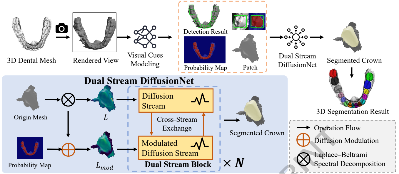
Figure 1: Overview of the proposed VGDM. Visual cues from a single rendered view are projected onto the mesh to modulate the Laplace-Beltrami operator, enabling a dual-stream diffusion architecture that suppresses cross-tooth feature leakage caused by spurious geometric connections.
