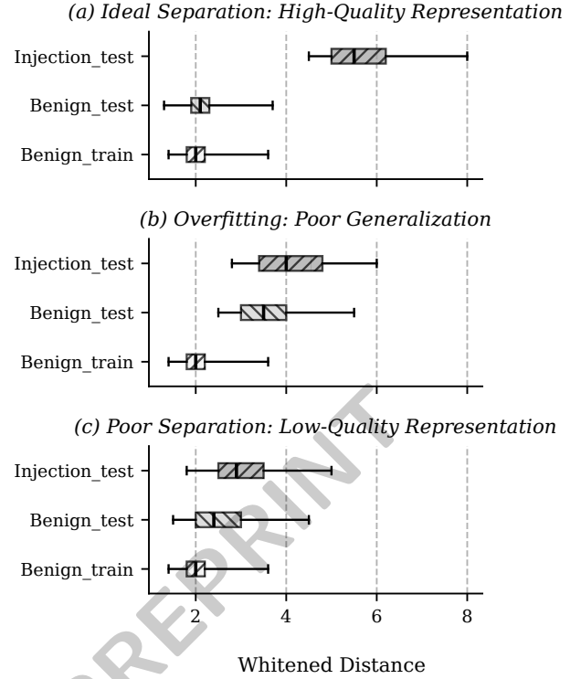
Figure 3: Interpreting model behavior with Whiten Distance Estimator (WIDE). Each panel illustrates how score distributions diagnose representation quality. (a) Successful learning: The benign and malicious clusters distribute distinctly apart. (b) Overfitting detected: Benign test samples are anomalously scored higher than their training counterparts, conflating with the adversarial cluster. (c) Model Collapse: The profound intermingling across datasets signals a collapse in learning, where the model fails to carve out distinguishable representations of the underlying manifolds.
