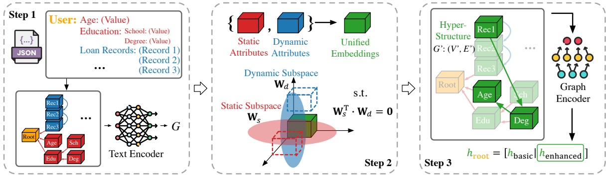
Figure 1: Overview of UniSAGE. Step 1: Construct a global attribute graph from JSON, with nodes as attributes/records and edges encoding hierarchical (static) and temporal (dynamic) relations. Step 2: Learn unified representations via orthogonal subspaces for non-interfering static aggregation and dynamic reasoning. Step 3: Capture task-specific cross-type interactions through a lightweight hyper-structure mechanism (SSAgg) to enhance downstream prediction.
