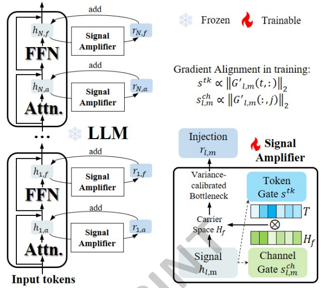
Figure 2: Overview of the signal amplifier for Noisy RAG. The amplifier reads post-module signals and selectively enhances them through token and channel gating. The combination of the carrier space and the variance-calibrated bottleneck ensures robust emphasis without overwhelming the model’s original representations. During training, the two-axis gating aligns naturally with gradient guidance, thereby ensuring the effectiveness of our approach.
