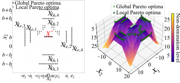
Figure 2: An instance of L1DM-2SIP (Definition 6) in the decision space, and its corresponding fitness landscape, shown by Pareto Landscape [Liang et al. , 2024].
