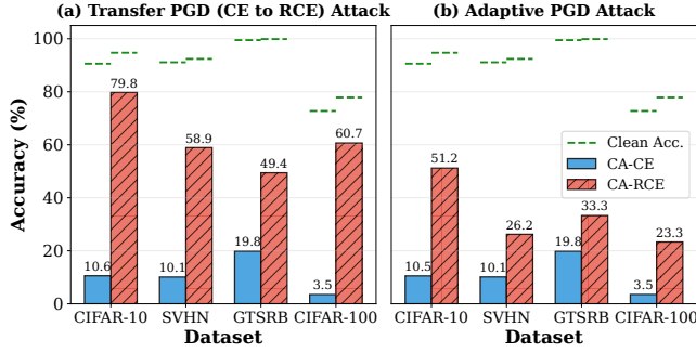
Figure 2: Robust accuracy comparison of CA-CE (blue) and CA-RCE (red) adapters under (a) transfer PGD attack crafted from CE model and (b) adaptive PGD attack crafted by their own loss functions. The dashed green line above each data is the clean accuracy of the corresponding model.
