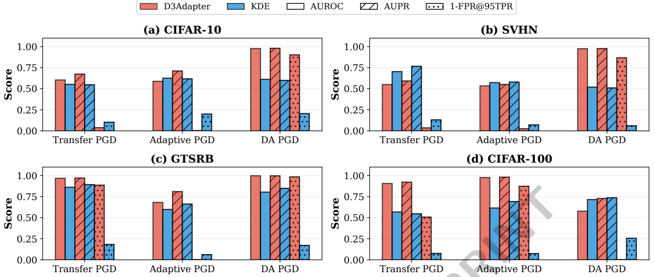
Figure 5: Detection performance comparison between D3Adapter and KDE across four datasets and three threat models. Bars show AUROC, AUPR, and 1 - \text{FPR}@95\text{TPR} (higher is better). Under detector-aware PGD, D3Adapter achieves AUROC gains of 0.37 on CIFAR-10, 0.46 on SVHN, and 0.19 on GTSRB compared to KDE, indicating that multi-adapter divergence is harder for the attacker to suppress than single-feature density. On transfer and adaptive PGD, the two methods perform comparably, with D3Adapter slightly ahead on CIFAR-10 and GTSRB and KDE slightly ahead on SVHN.
