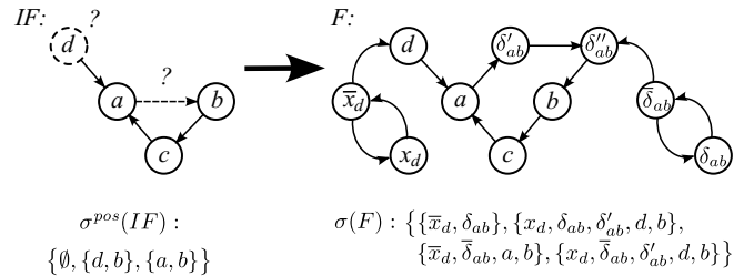
Figure 4: From an iAAF to a projection-equivalent AAF ( \sigma = \text{pr} )
