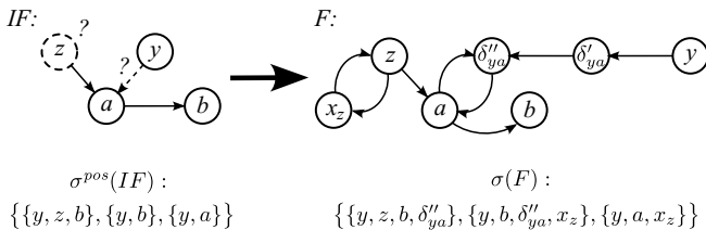
Figure 3: From an iAAF to a projection-equivalent AAF ( \sigma = \text{st} )
