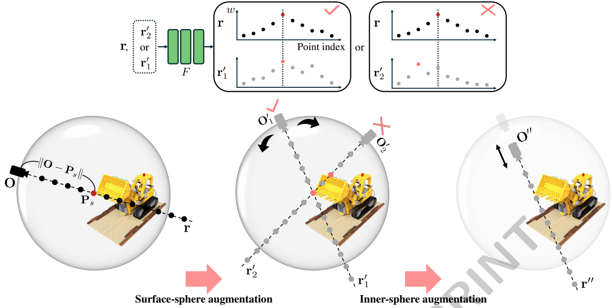
Figure 2: Overall structure of DivCon-NeRF. (Left) First, the virtual sphere is defined, centered at the predicted surface point P_s . (Center) A surface-sphere augmented ray r' is then cast from a randomly selected position on the sphere’s surface. (Right) To further enhance diversity, an inner-sphere augmented ray r'' is generated with a randomly selected radius within the sphere and the same random angle as the surface-sphere augmented ray. (Top) To maintain consistency, the consistency mask filters out inconsistent rays (e.g., r'_2 ) if the sampled point with the highest blending weight does not have the same index as the original.
