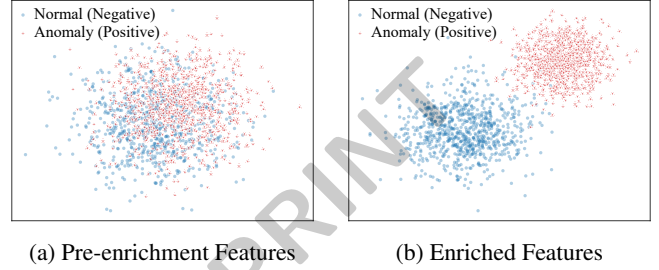
Figure 5: Feature visualization via t-SNE on UCF-Crime dataset.
