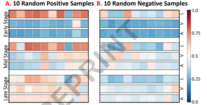
Figure 4: Similarity difference visualization between randomly sampled sentiment prototypes across training stages. Lighter colors indicate improved cross-modal alignment and more consistent sentiment representations.
