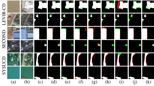
Figure 6: Qualitative results of different CD methods on LEVIR-CD, SECOND and SYSUCD datasets. (a) T1 Image, (b) T2 Image, (c) Ground Truth, (d) DTCDCSCN, (e) BIT, (f) Change Former, (g) ICIFNet, (h) DMINet, (i) USSFC-Net, (j) ChangeMamba, (k) Ours.
