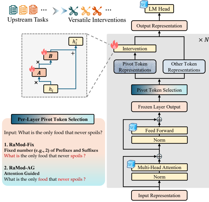
Figure 2: Our CTG framework RaMod consists of two stages. (i) In the first stage, we perform fine-tuning interventions separately for each upstream task. The intervention is applied at each layer to adapt the representations of pivot tokens. (ii) In the second stage, we generalize LLM with well-trained intervenes to unseen tasks. We propose a zero-shot intervention method for modular representation fine-tuning, enabling the model to adapt to unseen tasks effectively. Furthermore, we design an asynchronous orchestrator to dynamically allocate HBM as needed and proactively prune unnecessary interventions, thereby enhancing memory efficiency.
