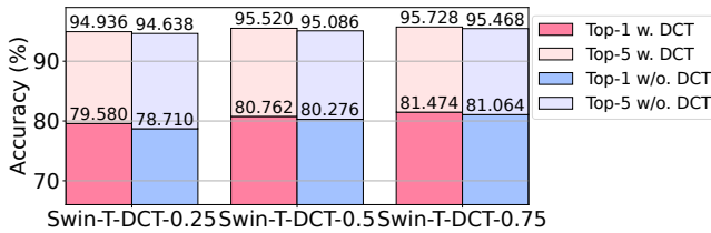
Figure 3: Ablation study on ImageNet-1K for removing DCT from DCT-compressed attention. Swin-T serves as the backbone model.
