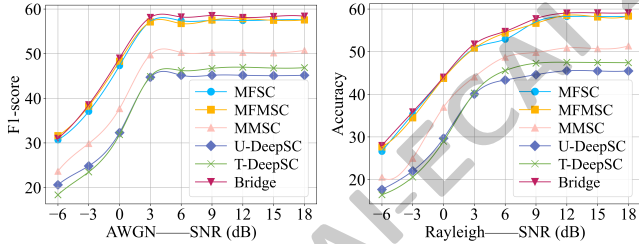
Figure 3: F1-score and accuracy performance of classification tasks.
