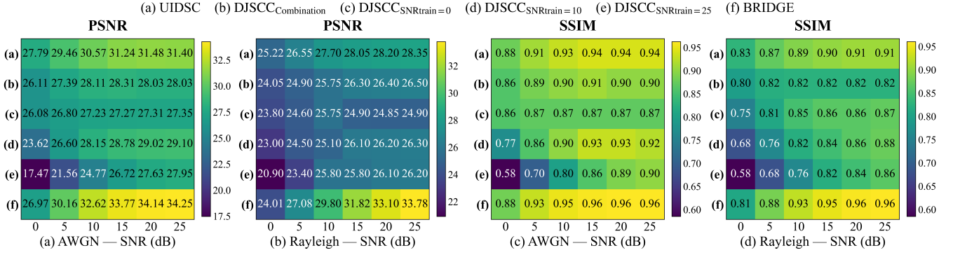
Figure 4: Reconstruction quality under different SNRs in AWGN and Rayleigh channels.
