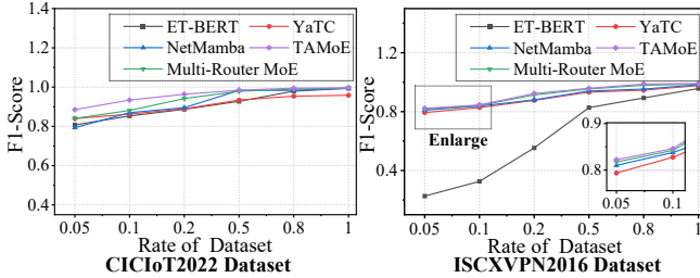
Figure 5: Model performance under different dataset proportions in the CICIoT2022 dataset and ISCXPVN2016 dataset.
