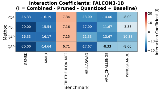
Figure 4: Interaction heatmap for Falcon3-1B-Base ( s = 0.2 ) across Q4P/PQ4 and Q8P/PQ8. TruthfulQA is the only benchmark with consistently positive I .
