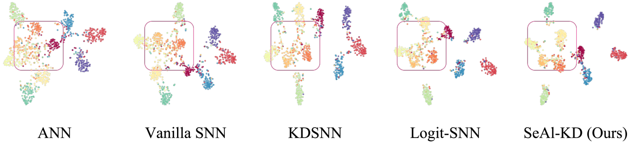
Figure 5: t-SNE visualization of learned feature representations on DVS-CIFAR10 under different direct-training and distillation methods.
