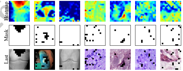
Figure 6: Mask visualization of FCM.
