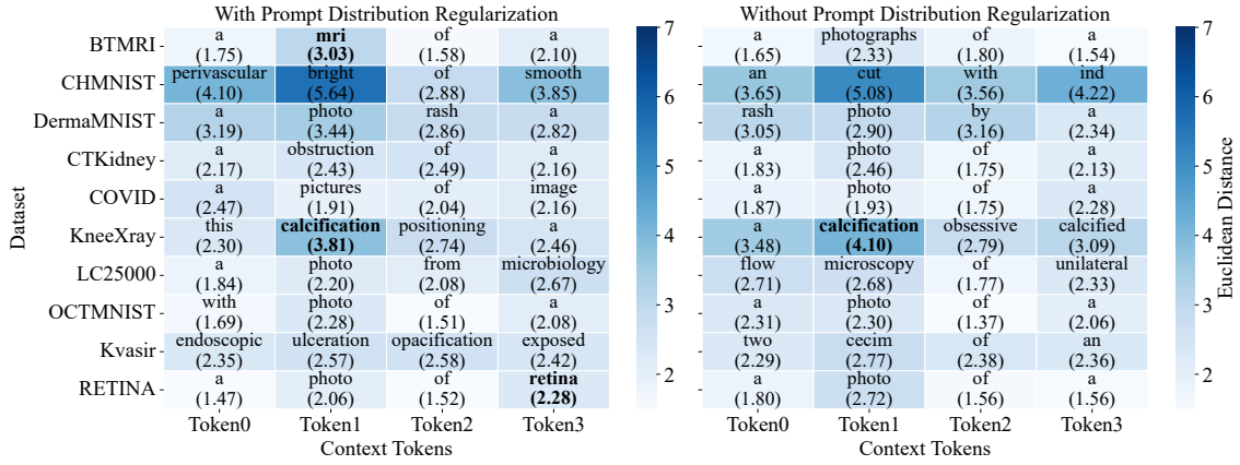
Figure 2: Visualization of the four nearest words for learned context tokens, with Euclidean distances in the embedding space.
