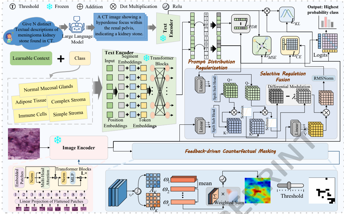
Figure 1: Overview of TriCLIP, a decomposition-driven and closed-loop calibration framework that stabilizes prompt conditioning, broadens visual evidence coverage, and enforces selective cross-modal fusion for robust biomedical vision–language classification.
