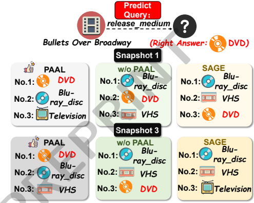
Figure 5: Case examples of PAAL.
