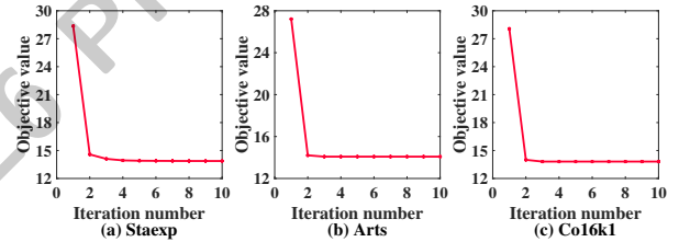
Figure 8: Convergence curves of EMMS on Staexp, Arts, and Co16k1 datasets.
