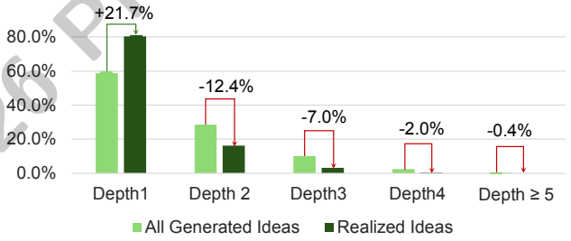
Figure 4: Depth-wise distribution of ideas before and after realization, showing that while ideas are generated across multiple hierarchical levels, realization is strongly biased toward shallow levels, with deeper ideas rarely instantiated.
