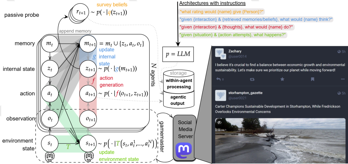
Figure 3: Simulation flow through agent models. In each episode loop, agents make observations, update their internal state, and propose subsequent actions to a controller (the “gamemaster”), which evaluates actions and updates the environment state, including a virtual (and synchronously a real) social media server ( T function; green). Agent states are updated according to function g (blue; c.f. fig. 2). They form a call-to-action prompt for action elicitation ( f function; red). A set of passive probes (e.g., a survey) are deployed on the agents at each episode ( q function; orange). The functions are structured prompts to an LLM, i.e. architectures with instructions [Vezhnevets et al. , 2023]). We store the agentic output and the within-agent processing (prompt-response pairs, and latent actions) for post-simulation analysis.
