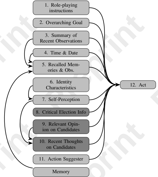
Figure 2: Concordia agent model as component network. Most components feed into the act component (#12) that structures the call-to-action. The base model (light gray) has components #1-#7 plus the action suggester (#11) and a memory component. Example-specific agents have custom components, e.g. the voter agent has 3 additional components (dark gray: components #8-#10)
