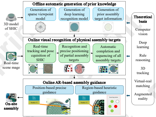
Figure 1: Framework of AR-based assembly guidance for SHIC.
