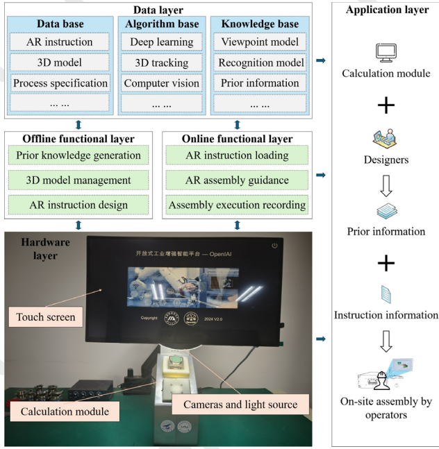
Figure 2: Structures of OpenIAI-SNIO.
