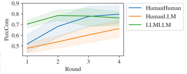
Figure 3: The average communicative performance ( PercCom ) per round across the conditions. Communication steadily increases over rounds except for the LLM-LLM condition, in which coordination happens in the first round but does not increase afterwards.
