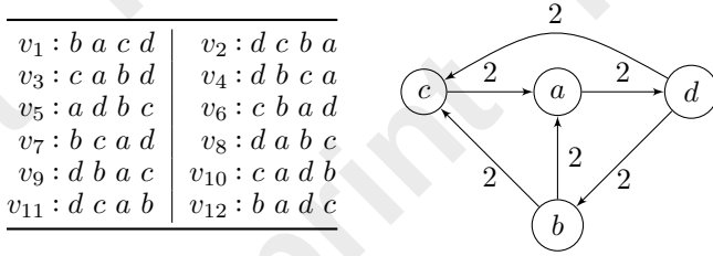
Figure 1: An election (left) and its WMG (right)
