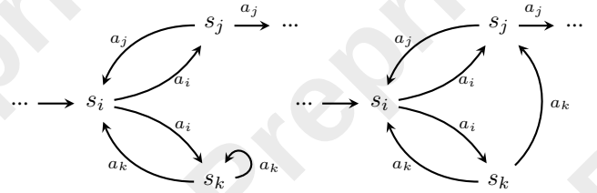
Figure 1: Two state transition graphs g_{\text{left}} and g_{\text{right}} , where s_i, s_j , and s_k are non-goal states, and a_i, a_j , and a_k are non-deterministic actions. The initial states s_0 are in the “...” leading to s_i .
