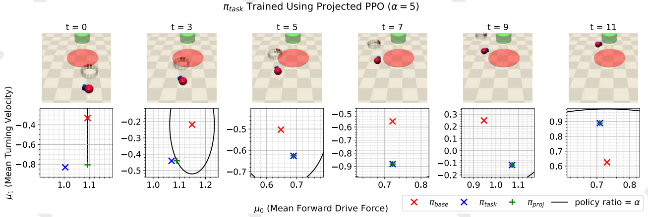
Figure 2: Snapshots across an example episode of the reach-avoid experiment using \pi_{proj} for Case 2 ( \pi_{task} trained using Projected PPO) and \alpha = 5 ; the bottom plots present the action means at the corresponding time step, with the black contour depicting the \alpha = 5 level set. Note that positive mean turning velocity represents anticlockwise rotation. The halo above the agent is a visualization of its LiDAR observations for the hazard and goal. See Appendix E.5 for Case 1 (pre-trained \pi_{task} ).
