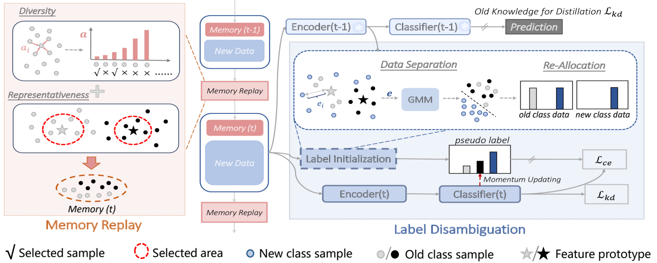
Figure 3: Overall framework of PGDR. The label disambiguation module divides new and old class samples based on prototypes and assigns different labels. PGDR then combines the momentum-updated pseudo-labels to achieve label disambiguation. After completing the task, the memory replay module is utilized to filter samples for subsequent training to mitigate forgetting.
