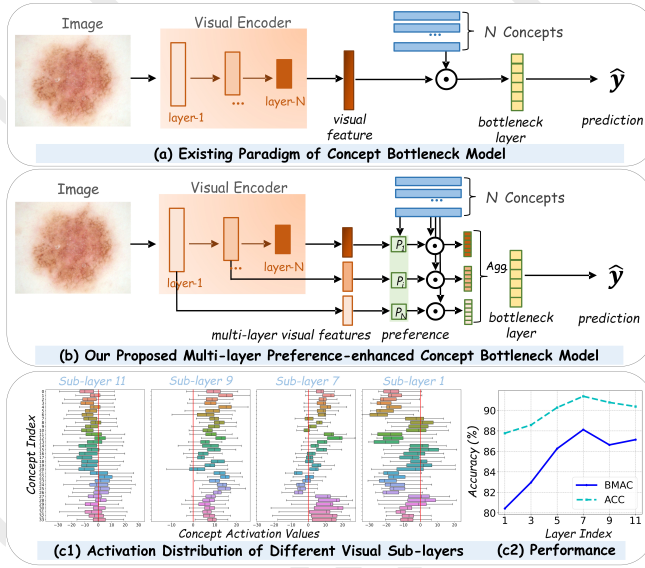
Figure 1: Illustration of our motivation. Unlike the existing CBM paradigm (Fig.a) that only uses features of the last standard layer of the visual encoder to correspond to concepts to explain the model’s prediction, we find that different visual sub-layer features exhibit varying preferences for concepts, i.e., some layer features are more inclined to activate and explain certain concepts, resulting in the default last standard layer may be not optimal (Fig.c). Thus, we propose to model the correspondence preference between visual sub-layer features and concepts, further comprehensively utilizing multi-layers to enhance the model’s interpretability and accuracy (Fig.b).
