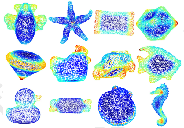
Figure 6: Visualization of our AGMA on Real3D-AD. AGAM extracts geometric variation information from the neighborhood of points, with regions colored in blue indicating gentle changes in geometric structure and areas colored in red exhibiting drastic changes.
