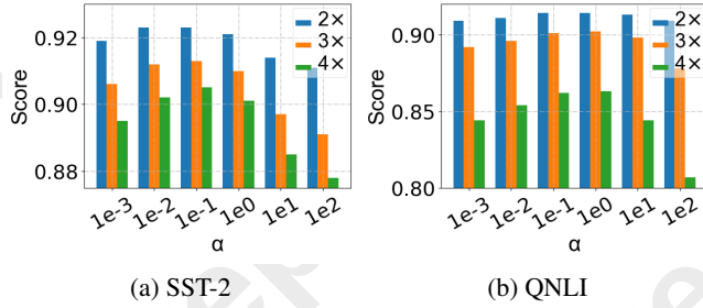
Figure 4: Impact of \alpha on the task performance under different speed-up ratios for SST-2 and QNLI tasks.
