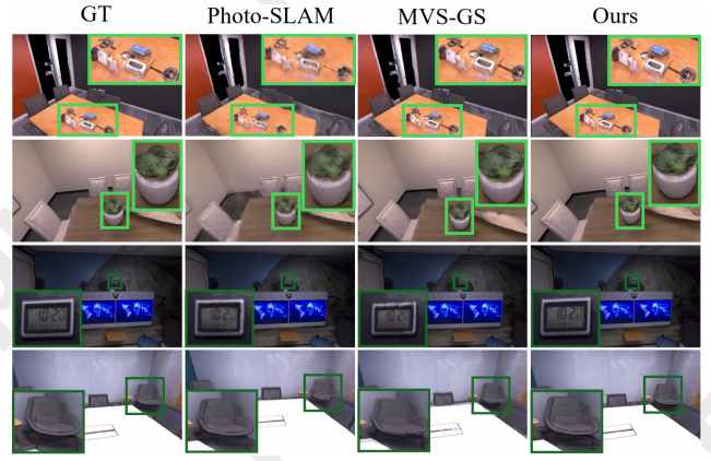
(a) Results on the Replica dataset
