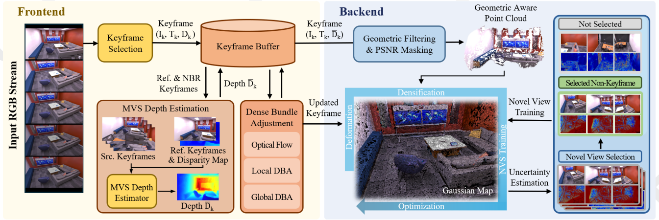
Figure 2: System overview. The frontend tracks camera poses and estimates depth maps for keyframes using MVS networks, with the disparity map derived from tracking module used to initialize the network. The backend generates new Gaussians from keyframes and continuously optimizes the 3DGS model. To further improve performance, our system periodically performs GBA and conducts additional training on non-keyframes selected through NVS.
