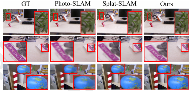
(b) Results on the TUM-RGBD dataset
