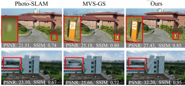
(a) Results on the Aerial dataset
