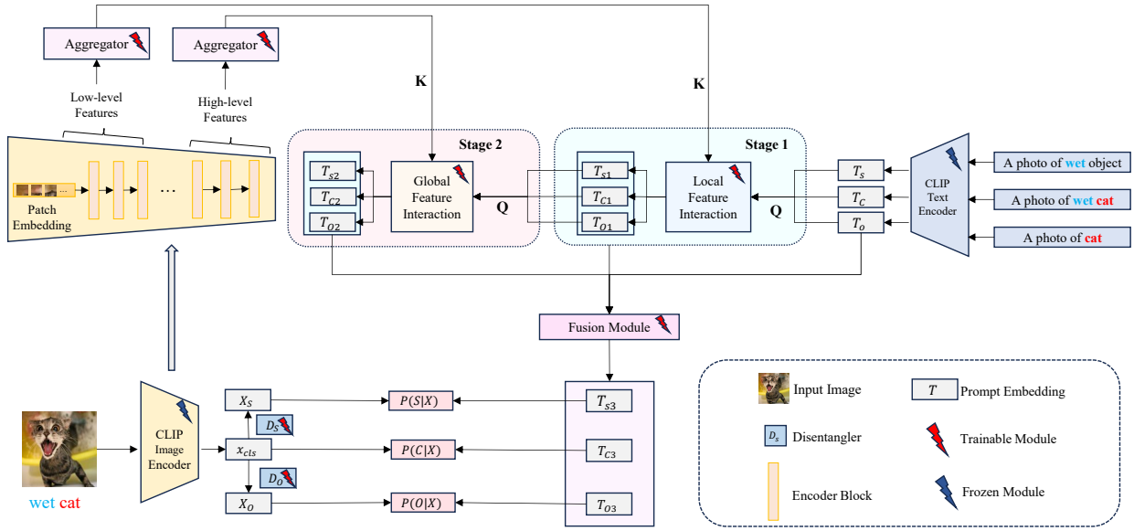
Figure 2: The general framework of the MSCI model. We design two self-adaptive aggregators to extract local and global visual information from low-level and high-level visual features, respectively, and integrate this information into the prompt embeddings through stage-wise cross-modal interactions. Additionally, a fusion module is introduced to regulate the influence of local and global information on the generation of the final prompt embeddings.
