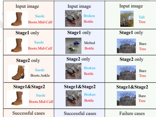
Figure 5: Qualitative analysis of the proposed model.
