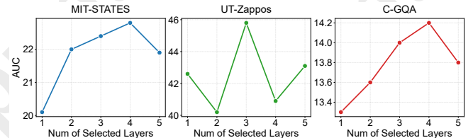
Figure 4: The impact of the number of aggregated layers N on AUC.
