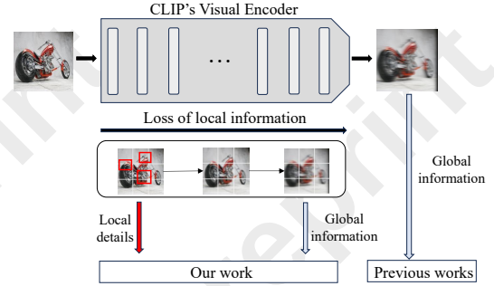
Figure 1: Core idea of our work. By effectively leveraging the rich local details in the lower-level features of the visual encoder, CLIP’s ability to capture fine-grained local information can be enhanced.
