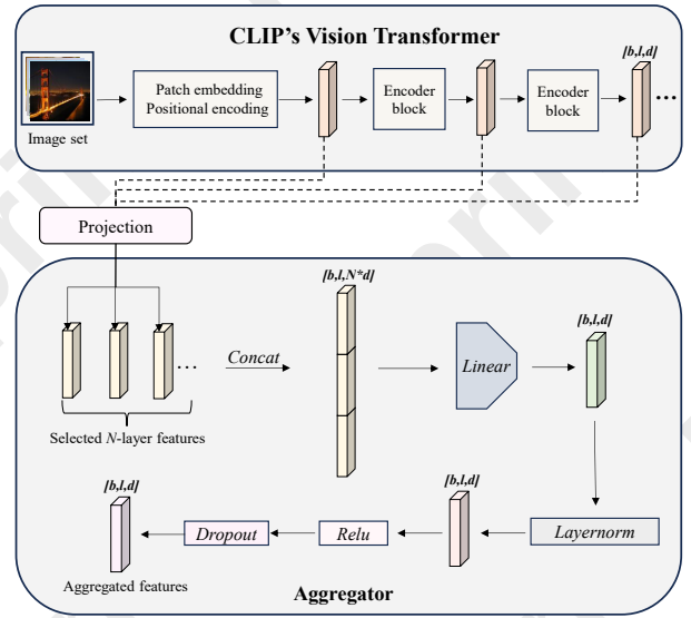
Figure 3: Illustration of the low-level feature aggregator.
