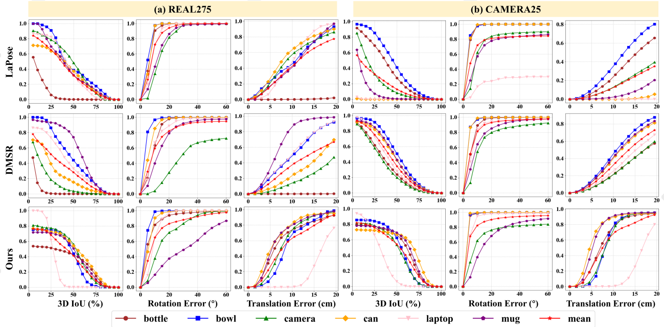
Figure 3: AP curves in terms of different types of errors on (a) REAL275 and (b) CAMERA25 datasets.
