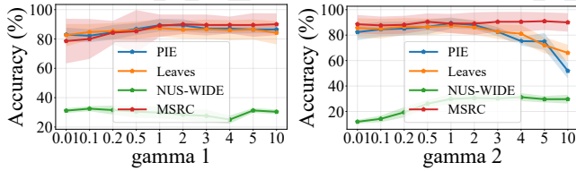
Figure 4: Classification accuracy (%) on four datasets with different \gamma_1 (gamma 1) and \gamma_2 (gamma 2) (one random view is attacked).
