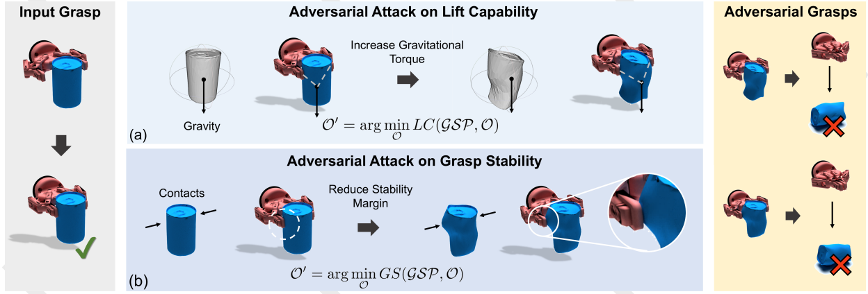
Figure 2: Illustration of AdvGrasp: Given a 3D object and its corresponding grasp configuration as inputs, AdvGrasp deforms the object in two key ways: (a) increasing gravitational torque to weaken lift capacity and (b) reducing the stability margin in the wrench space to compromise grasp stability, ultimately leading to grasp failure.
